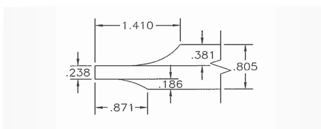
Cove Full Thickness Panel
