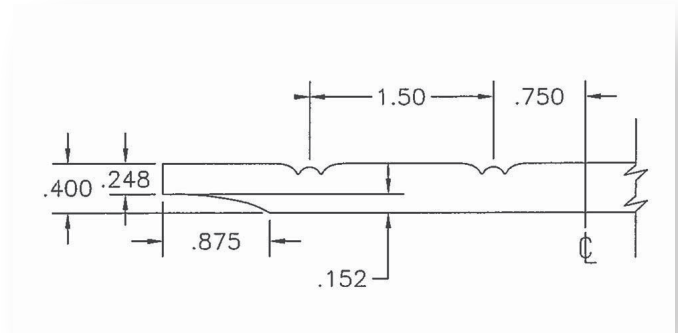
Reverse Beaded Panel
