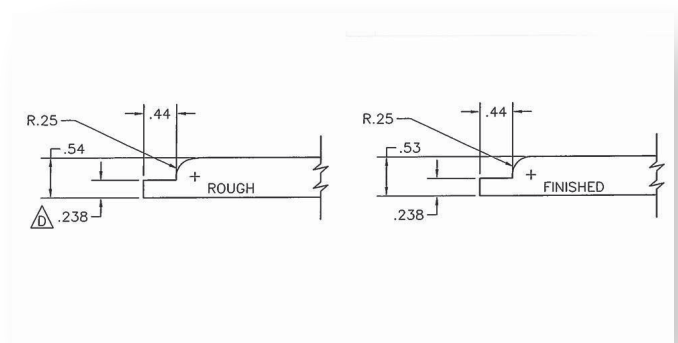
Round Over Full Thickness Panel
