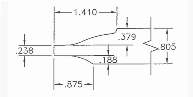
Ogee Full Thickness Panel
