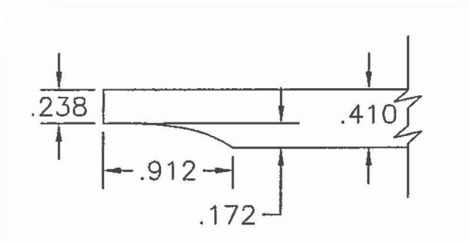
Reverse Raised Panel
