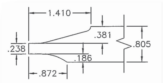
15 Degree Full Thickness Panel
