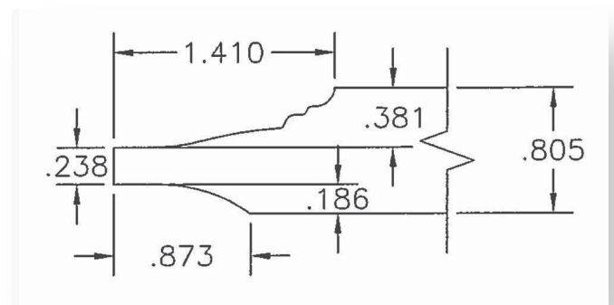
Cove & Bead Full Thickness Panel
